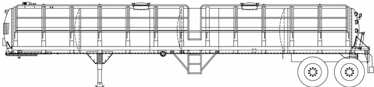
Standard 6300 Gallon / 62" Diameter Heads / Optional Grip Strut Walkway Totally Enclosed
